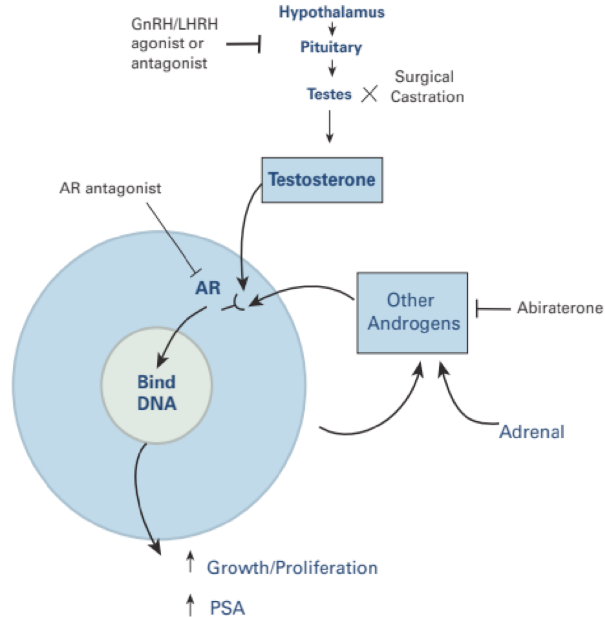
Fig. 14-4. Basic schematic of androgen receptor-directed therapies.
