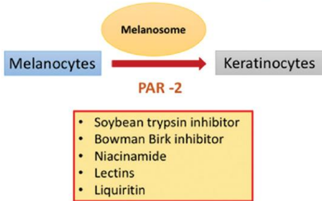
Figure 4: Role of a defective skin barrier in melisma
